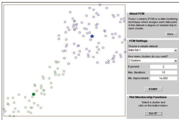
Figure 2: 2D Image data point in the data set a degree of membership to each cluster.
